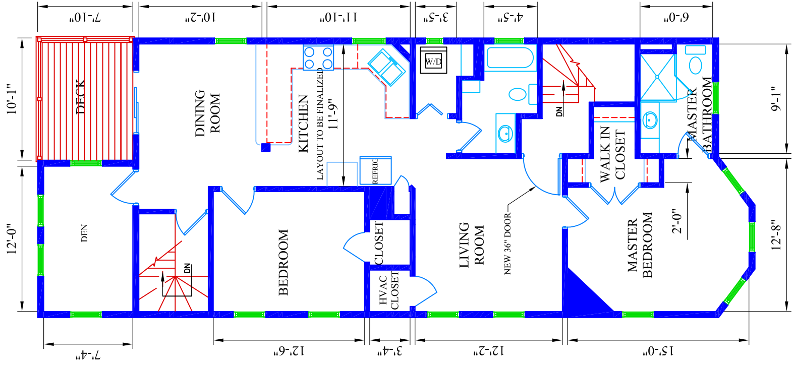
PROPOSED THIRD FLOOR PLAN
